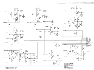
UHF 4 Channel Model Controller_3D Schematic Diagram 2 of 2
