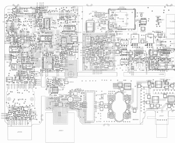
UHF Main Board Component Side PCB No. 8402624Y0
