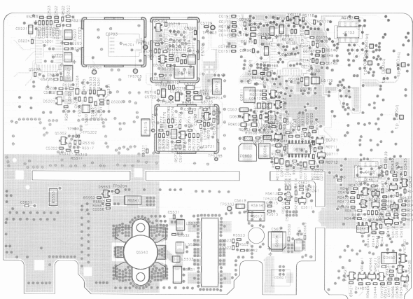
UHF Main Board Solder 5
