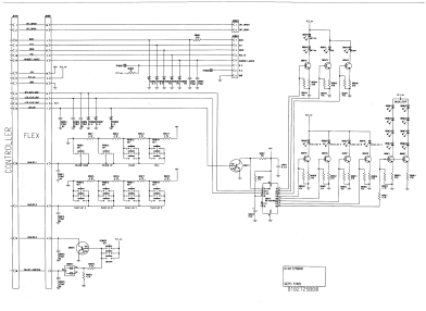
Control Head X Schematic Diagram
