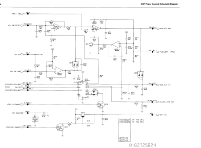
UHF Power Control Schematic Diagram
